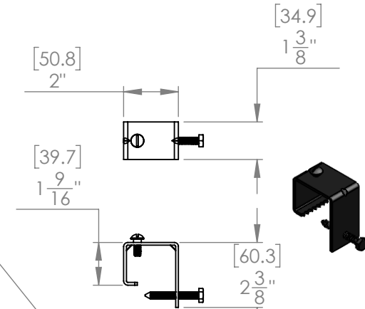
BRACKET SUB-ASSEMBLY SCALE 1:5 Removed for packing
